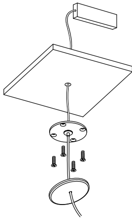
Ceiling Plate Ø76 x 8mm
